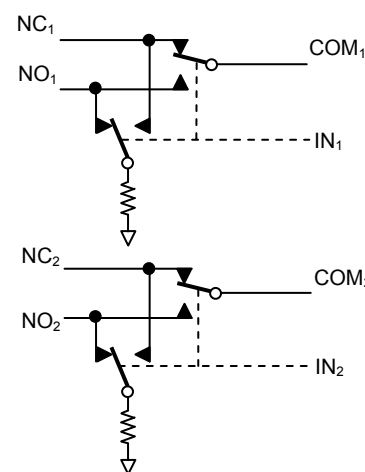
Fig.2 PA2268T (with termination resistors)
