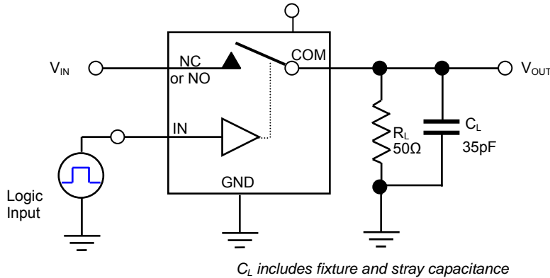
Figure 1. AC Test Circuit
