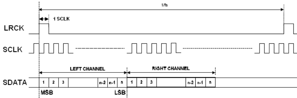
Figure 7 DSP/PCM Mode B
