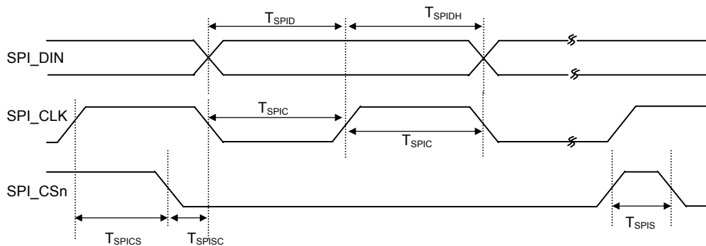
Fig.9 Serial Control Port SPI Timing
